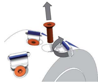
The body of the Stehle DP Jointing Cutterhead is reusable. Damaged cutting edges can be exchanged individually.
